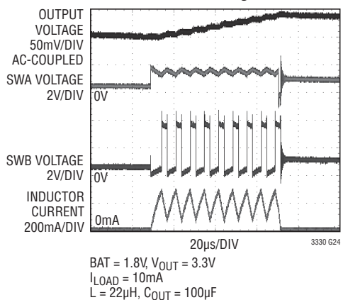
Buck-Boost Switching Waveforms
