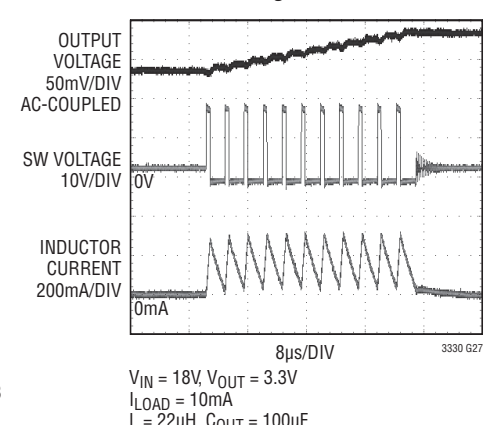
Buck Switching Waveforms
